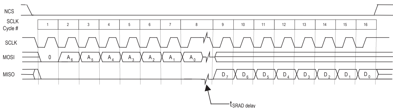
Figure 18. Read Operation
