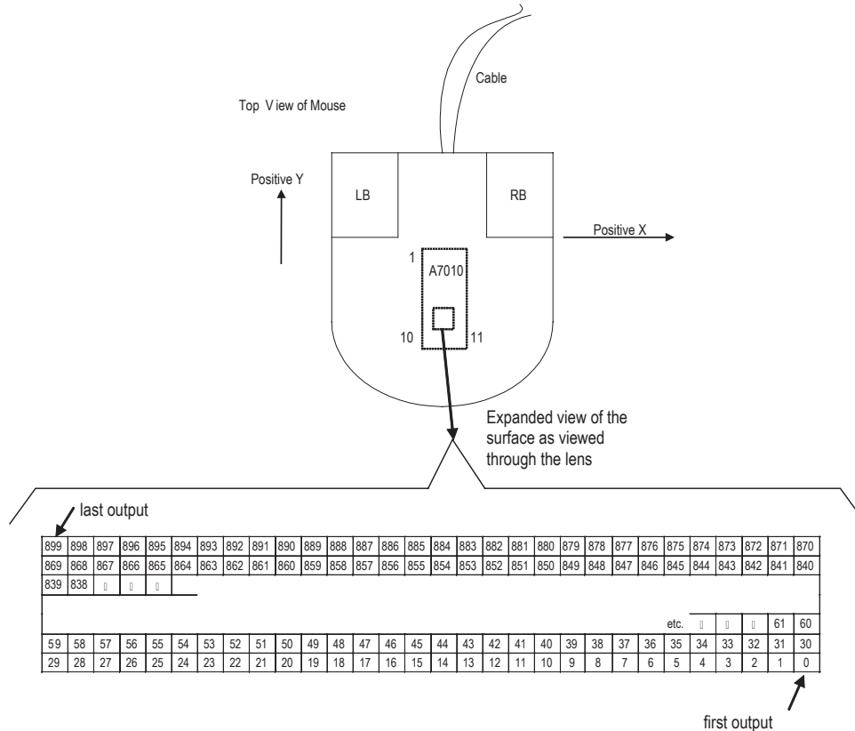
Figure 26. Pixel address map of navigation surface image (Sensor looking at the navigation surface through the ADNS-6120 lens from the top of mouse)
