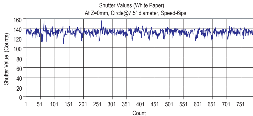
Figure 29. Shutter Values at 1600dpi (White Paper)
