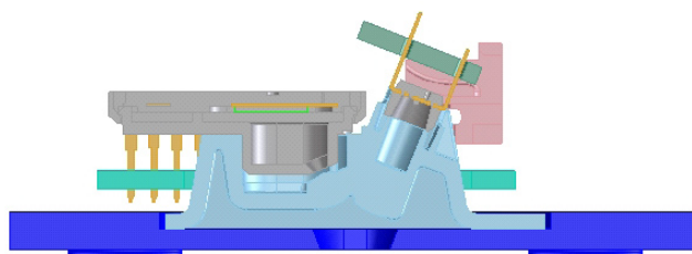
Figure 6. Cross section of PCB assembly
