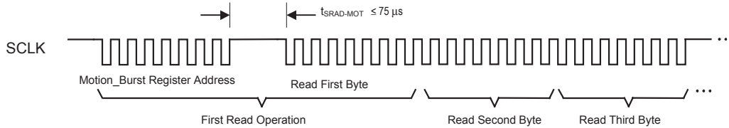
Figure 23. Motion burst timing.
